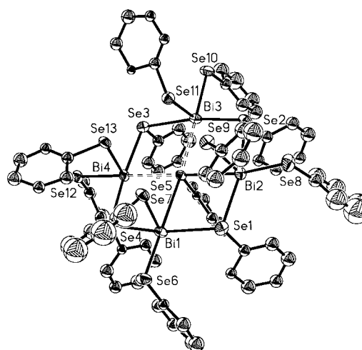
Fig. 1 The molecular structure of [\text{Bi}_4(\mu\text{-SePh})_5(\text{SePh})_8]^- 1 (molecule 1), isolated as its [\text{HP}^*\text{Pr}_3]^+ salt, illustrating the near planar arrangement of the four Bi and five \mu\text{-Se} centres. Selected bond lengths (Å) and angles (°): \text{Se-C} 1.87(3)–1.98(3), \text{Bi1-Se7} 2.657(3), \text{Bi1-Se6} 2.731(3), \text{Bi1-}\mu\text{-Se} 2.890(3)–3.248(3), \text{Bi2-Se9} 2.646(4), \text{Bi2-Se8} 2.737(4), \text{Bi2-}\mu\text{-Se} 2.974(3)–3.277(3), \text{Bi3-Se11} 2.649(3), \text{Bi3-Se10} 2.696(3), \text{Bi3-}\mu\text{-Se} 2.984(4)–3.312(3), \text{Bi4-Se13} 2.655(3), \text{Bi4-Se12} 2.696(3), \text{Bi4-}\mu\text{-Se} 2.962(3)–3.337(3); \text{Bi1-Se1-Bi2} 99.62(8), \text{Bi1-Se5-Bi2} 92.4(1), \text{Se6-Bi1-Se7} 93.0(1), \text{Bi1-Se7-C} 102.5(10), \text{Se1-Bi1-Se7} 86.4(1), \text{Se1-Bi2-Se9} 91.8(1), \text{Se1-Bi2-Se2} 167.7(1), \text{Se2-Bi3-Se3} 167.7(1), \text{Se3-Bi4-Se4} 168.88(9), \text{Se1-Bi1-Se4} 170.11(9).
