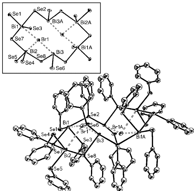
Fig. 2 The molecular structure of [\text{Bi}_6(\mu\text{-SePh})_6(\text{SePh})_{10}\text{Br}_2] 2 . Selected bond lengths (Å) and angles (°): Bi1–Se1 2.670(2), Bi1–Se3 2.703(2), Bi1–μ-Se2 3.110(2), Bi1–μ-Se7 2.820(2), Bi1–Br1 3.279(2), Bi2–Se4 2.650(2), Bi2–Se5 2.663(2), Bi2–μ-Se7 3.009(2), Bi2–μ-Se8 2.999(2), Bi2–Br1 3.336(2), Bi3–Se6 2.666(2), Bi3–Se8 2.774(2), Bi2–μ-Se2A 2.767(2), Bi2–Br1 3.269(2); Se1–Bi1–Se3 101.34(6), Se1–Bi1–Se7 88.84(6), Se3–Bi1–Se7 80.41(5), Se1–Bi1–Se2 85.08(5), Se3–Bi1–Se2 79.60(5), Se7–Bi1–Se2 157.50(5), Se4–Bi2–Se5 93.11(6), Se4–Bi2–Se8 89.53(5), Se5–Bi2–Se8 95.19(6), Se4–Bi2–Se7 98.12(5), Se5–Bi2–Se7 91.87(6), Se8–Bi2–Se7 169.30(5), Se6–Bi3–Se2A 189.31(6), Se6–Bi3–Se8 87.46(5), Se2A–Bi3–Se8 91.30(5), Bi3A–Se2–Bi1 92.65(5), Bi1–Se7–Bi2 94.63(5), Bi3–Se8–Bi2 101.26(5).
